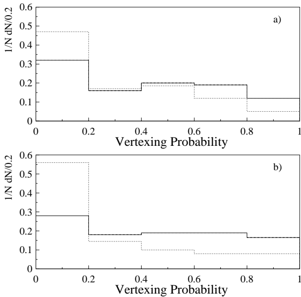
Fig. 21. Probability of the lepton- X_{ch} vertex with: a no cut on NN_{bu} , b NN_{bu} > 0.8 . Comparison between simulated b \rightarrow X_c l \nu_e (dotted line) and b \rightarrow u (solid line) transitions
