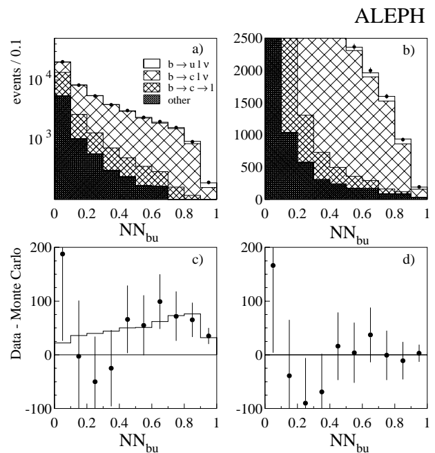
Fig. 10. Neural network output NN_{bu} : a and b comparison between data ( points ) and Monte Carlo ( histogram ), c difference between data and Monte Carlo with no b \rightarrow u transitions ( points ) compared to the b \rightarrow u contribution ( histogram ), and d difference between data and Monte Carlo with the fitted value of b \rightarrow u
