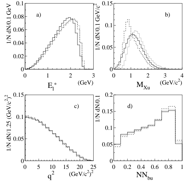
Fig. 13. a Lepton momentum, b hadronic invariant mass, c q^2 of the virtual W for signal events as predicted by completely inclusive models: DSU model ( solid lines ), ACCMM model ( dashed lines ) and the parton model ( dotted lines ). d shows the effect of the inclusive modelling on the NN_{bu} output obtained with the hybrid model using \Lambda = 1.6 GeV and ISGW2 for the exclusive part
