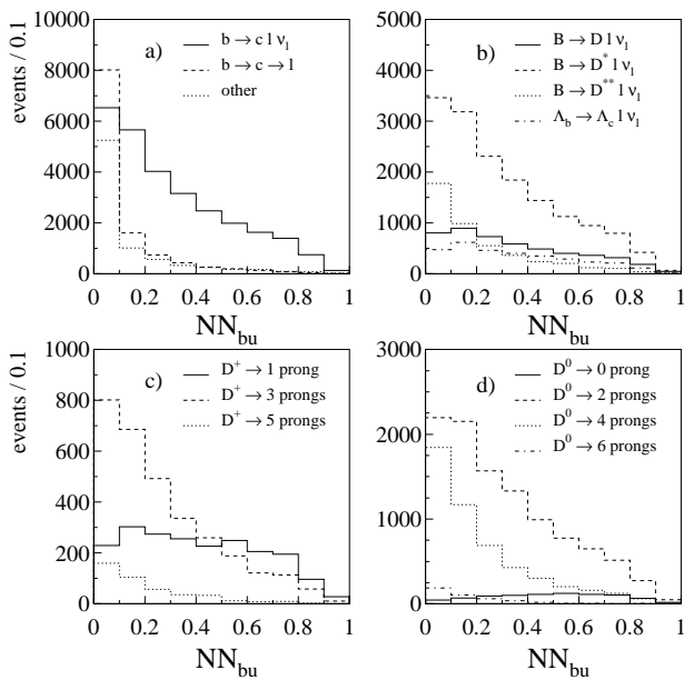
Fig. 7a–d. Breakdown of the b \rightarrow c background into its main components. a Comparison between direct b \rightarrow c l \nu_\ell and cascade b \rightarrow c \rightarrow \ell transitions, b comparison between different hadronic final states X_c , c and d comparison of topological final states in D^+ and D^0 decays respectively. The histograms are normalized to the number of entries used in the fit of the data. In a , “other” includes non prompt leptons from b decays, leptons from \psi and \tau decays and the small contribution from Z decays into light quarks
