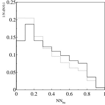
Fig. 11. Output of NN_{bu} for simulated A_c decays with ( solid line ) and without ( dotted line ) a neutron in the final state. The two contributions are normalized to the same area
