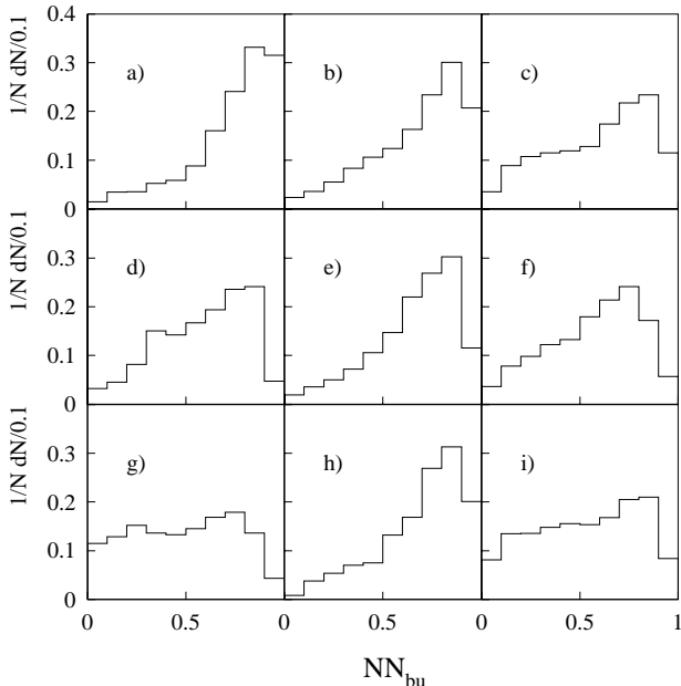
Fig. 8. Output of NN_{bu} for simulated b \rightarrow X_u l \nu_\ell transitions: a B \rightarrow \pi^0 l \nu_\ell , b B \rightarrow \pi^+ l \nu_\ell , c B \rightarrow (\eta + \eta') l \nu_\ell , d B \rightarrow \rho^0 l \nu_\ell , e B \rightarrow \rho^+ l \nu_\ell , f B \rightarrow \omega l \nu_\ell , g B \rightarrow (f + a + b) l \nu_\ell + B_s \rightarrow K^{**} l \nu_\ell , h B_s \rightarrow (K + K^*) l \nu_\ell , i b \rightarrow (n\text{-body}) l \nu_\ell . The different contributions are normalized to the same area
