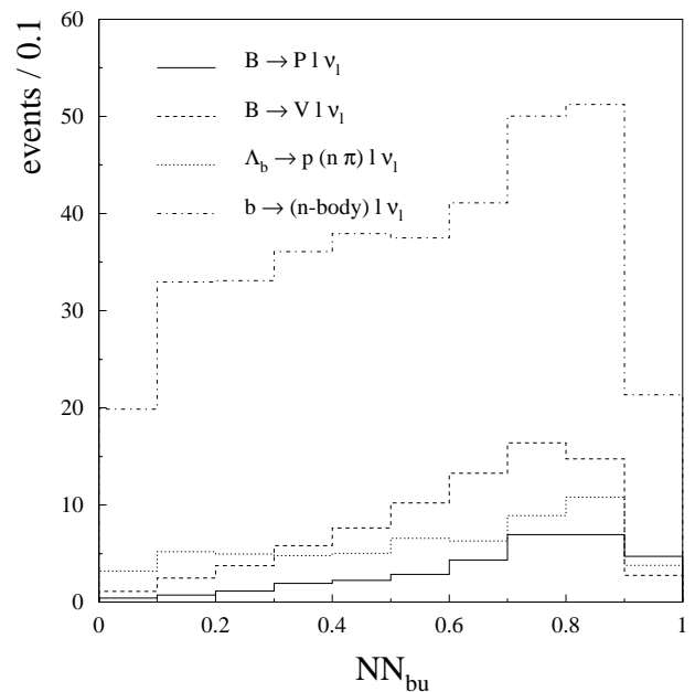
Fig. 9. Breakdown of the b \rightarrow X_u l \nu_\ell contribution into resonant pseudoscalar (P) and vector (V) states, nonresonant b meson decays and \Lambda_b decays. The histograms are normalized to the fitted value of \text{Br}(b \rightarrow X_u l \nu_\ell) and the hybrid model described in Sect. 4.2 is used
