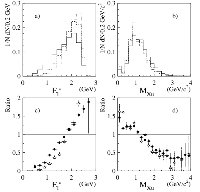
Fig. 12. a Lepton energy distribution in the b hadron centre-of-mass frame, b invariant mass of the hadronic system obtained in b \rightarrow u\ell\nu_\ell transitions with a cut on NN_{bu} at 0.0 ( solid lines ), 0.6 ( dashed lines ) and 0.8 ( dotted lines ), c (resp. d ) shows the ratio of histogram a (resp. b ) with cut at 0.6 ( points ) and 0.8 ( triangles ) to the histogram with no cut
